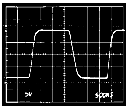
Figure 24. Pulse Response of the 3 Op Amp Instrumentation Amplifier. Gain = 10, Horizontal Scale: 0.5 \mu\text{s}/\text{Div} , Vertical Scale: 5 \text{ V}/\text{Div} .
