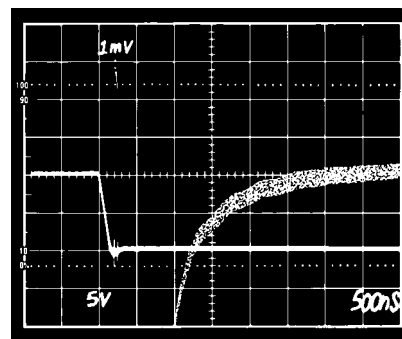
Figure 25. Settling Time of the 3 Op Amp Instrumentation Amplifier. Gain = 10, Horizontal Scale: 0.5 \mu\text{s}/\text{Div} , Vertical Scale: 5 \text{ V}/\text{Div} . Error Signal Scale: 0.01\%/\text{Div} .
