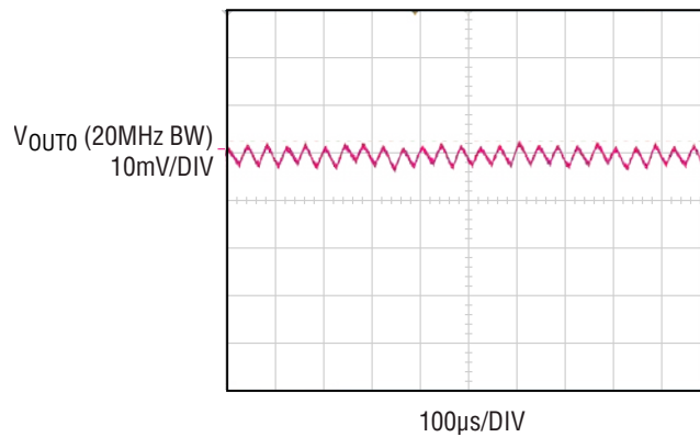
Figure 7. V OUT0 Voltage Ripple at V IN = 48V, V OUT0 = 1.0V, I OUT0 = 50A
