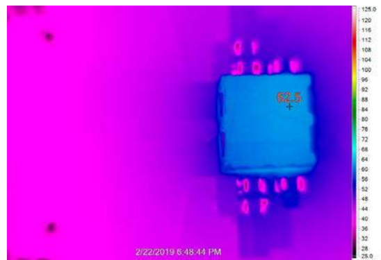
Figure 8. Thermal at V IN = 48V, V OUT0 = 1.0V, I OUT0 = 50A, T A = 25°C, No Airflow
