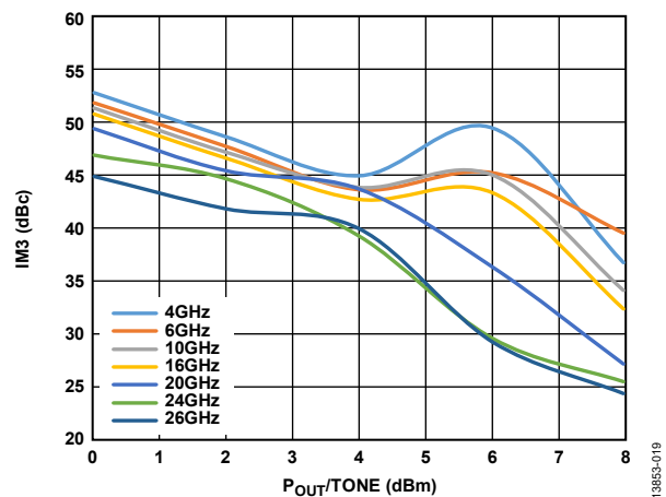
Figure 19. Output Third Order Intermodulation (IM3) vs. P_{OUT/Tone} for Various Frequencies at V_{DD} = 6 \text{ V}
