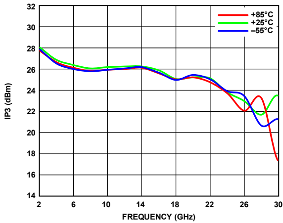
Figure 16. Output IP3 vs. Frequency for Various Temperatures at P_{OUT} = 0 \text{ dBm/Tone}
