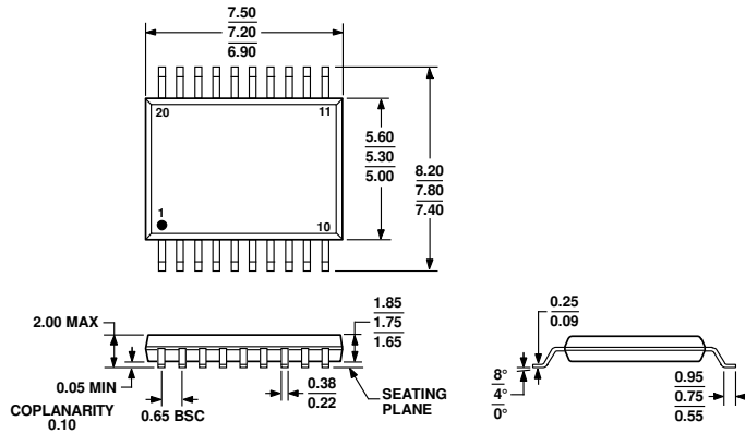
Figure 22. 20-Lead Shrink Small Outline Package [SSOP] (RS-20)
