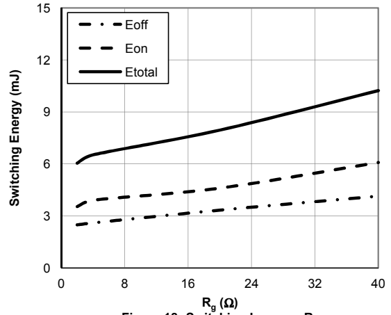
Figure 18: Switching Loss vs. R_g ( T_J=175^\circ\text{C} , V_{GE}=15\text{V} , V_{CE}=400\text{V} , I_C=75\text{A} )
