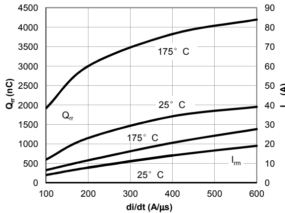
Figure 23: Diode Reverse Recovery Charge and Peak Current vs. di/dt ( V_{GE}=15V, V_{CE}=400V, I_F=75A )
