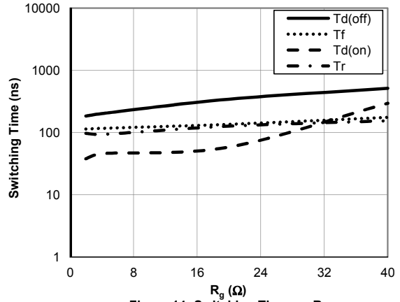
Figure 14: Switching Time vs. R_g ( T_J=175^\circ\text{C} , V_{GE}=15\text{V} , V_{CE}=400\text{V} , I_C=75\text{A} )
