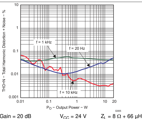
Figure 5. Total Harmonic Distortion + Noise vs Output Power
