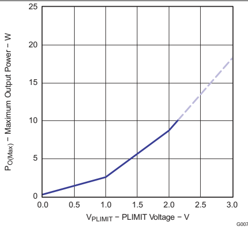
Dashed line represents thermally limited region. Gain = 20 dB V_{CC} = 24\text{ V} Z_L = 8\ \Omega + 66\ \mu\text{H}
