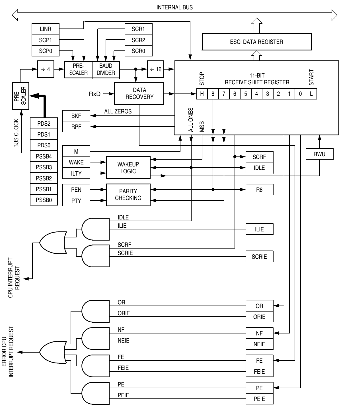
Figure 15-6. ESCI Receiver Block Diagram
