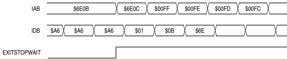
Figure 16-16. Wait Recovery from Interrupt
