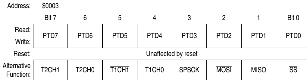
Figure 13-13. Port D Data Register (PTD)
