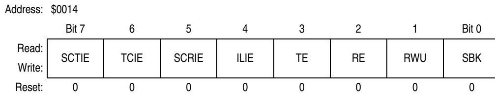
Figure 15-11. ESCI Control Register 2 (SCC2)
