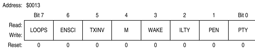
Figure 15-10. ESCI Control Register 1 (SCC1)
