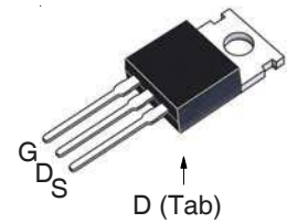
TO-220 (IXTP)
