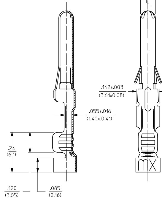
SECTION "C-C"
