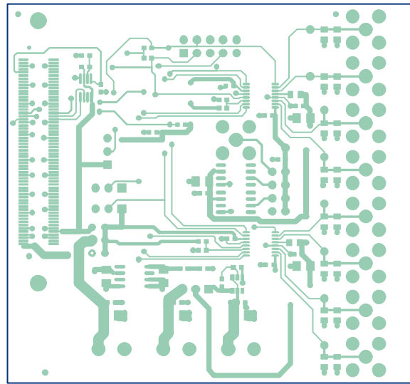
Figure 8. AD569x(R) Top Side Routing
