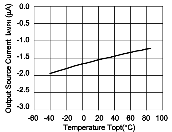
12) Output Source Current vs. Temperature R1282D002A
