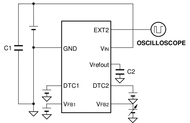
Test Circuit 4
