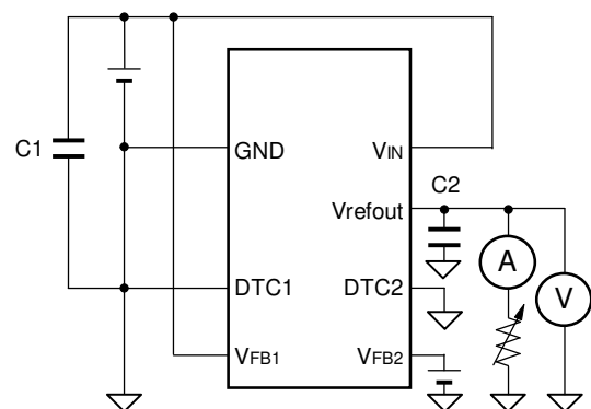
Test Circuit 6
