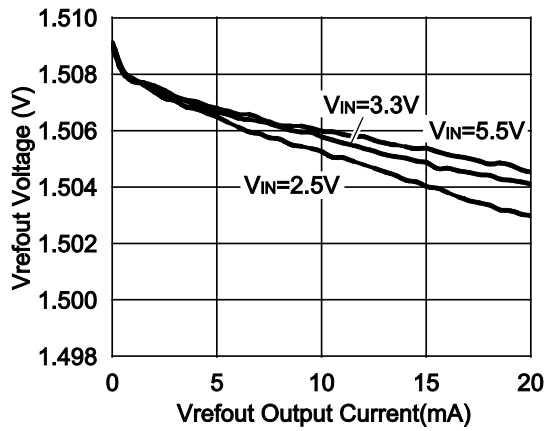
8) Vrefout Output Voltage vs. Output Current R1282D002A
