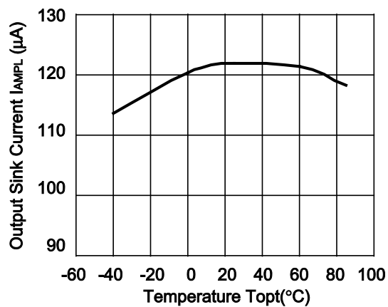
11) Output Sink Current vs. Temperature (V IN =3.3V) R1282D002A
