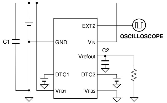
Test Circuit 2
