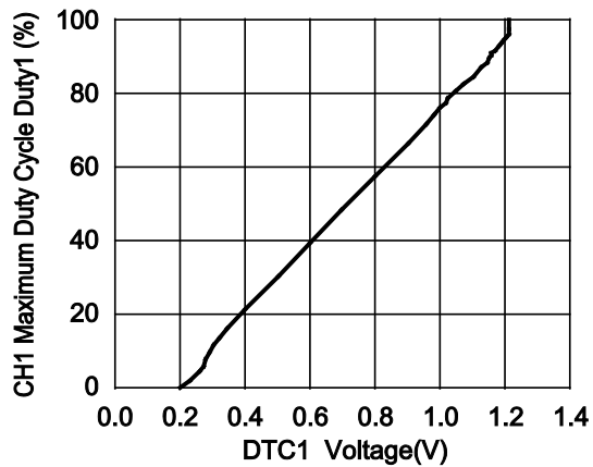
10) Maximum Duty Cycle vs. DTC Voltage (V IN =3.3V) R1282D002A
