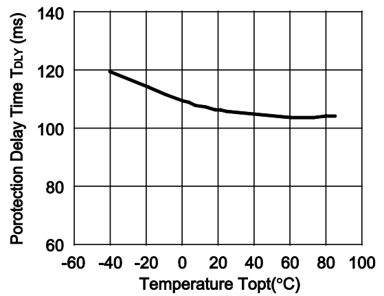
9) Protection Delay Time vs. Temperature (V IN =3.3V) R1282D002A
