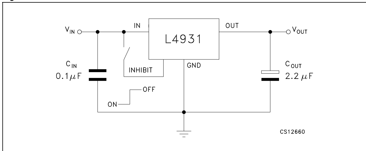
Figure 3. Test circuits
