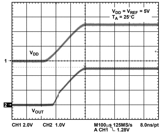
Figure 32. Power-On Reset to Midscale
