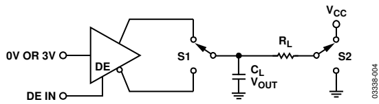
Figure 3. Driver Voltage Measurement Test Circuit
