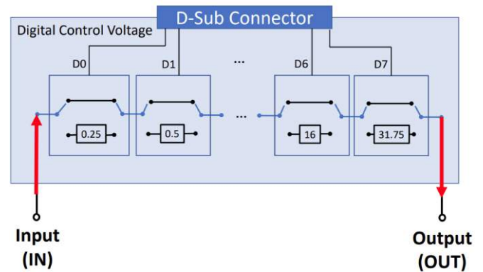
Electrical Schematic
