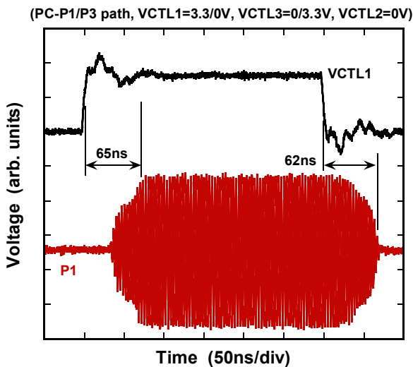
Switching Time
