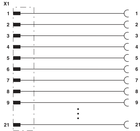
Circuit diagram
