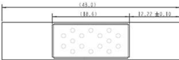
Front View (Component Side)
