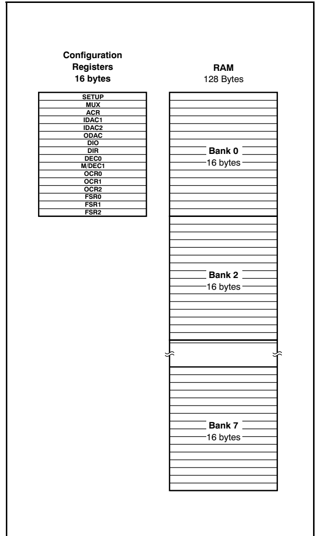
Figure 29. Memory Organization
