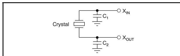
Figure 26. Crystal Connection
