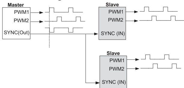
Figure 4: Block Diagram of Master-Slave Synchronization Connection
