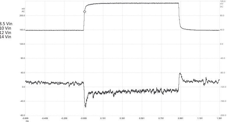
Top Trace: Load Current Bottom Trace: Output Voltage (40 mV / div) Slew Rate: (1A/ \mu s) Current step-change (6.25-18.75-6.25 A) Time Scale: (200 \mu s / div)
