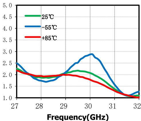
VSWRo(:1) vs.Temperature
