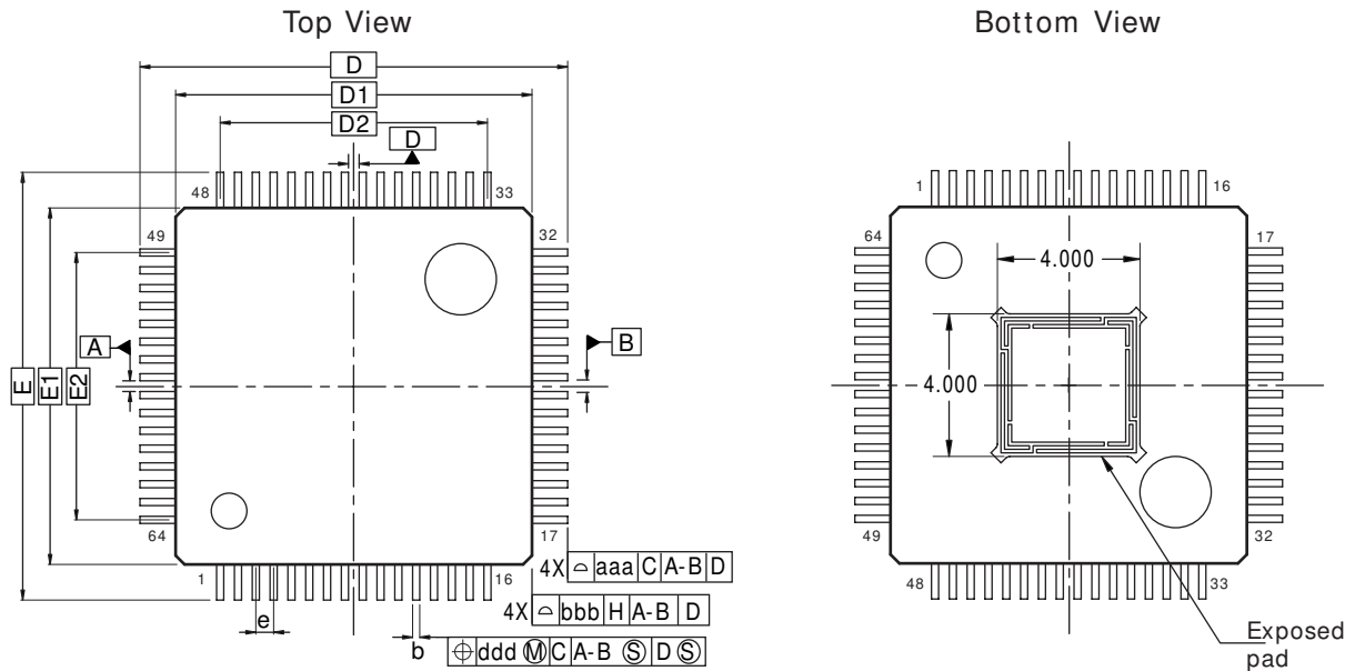
Figure 24. Package Drawing
