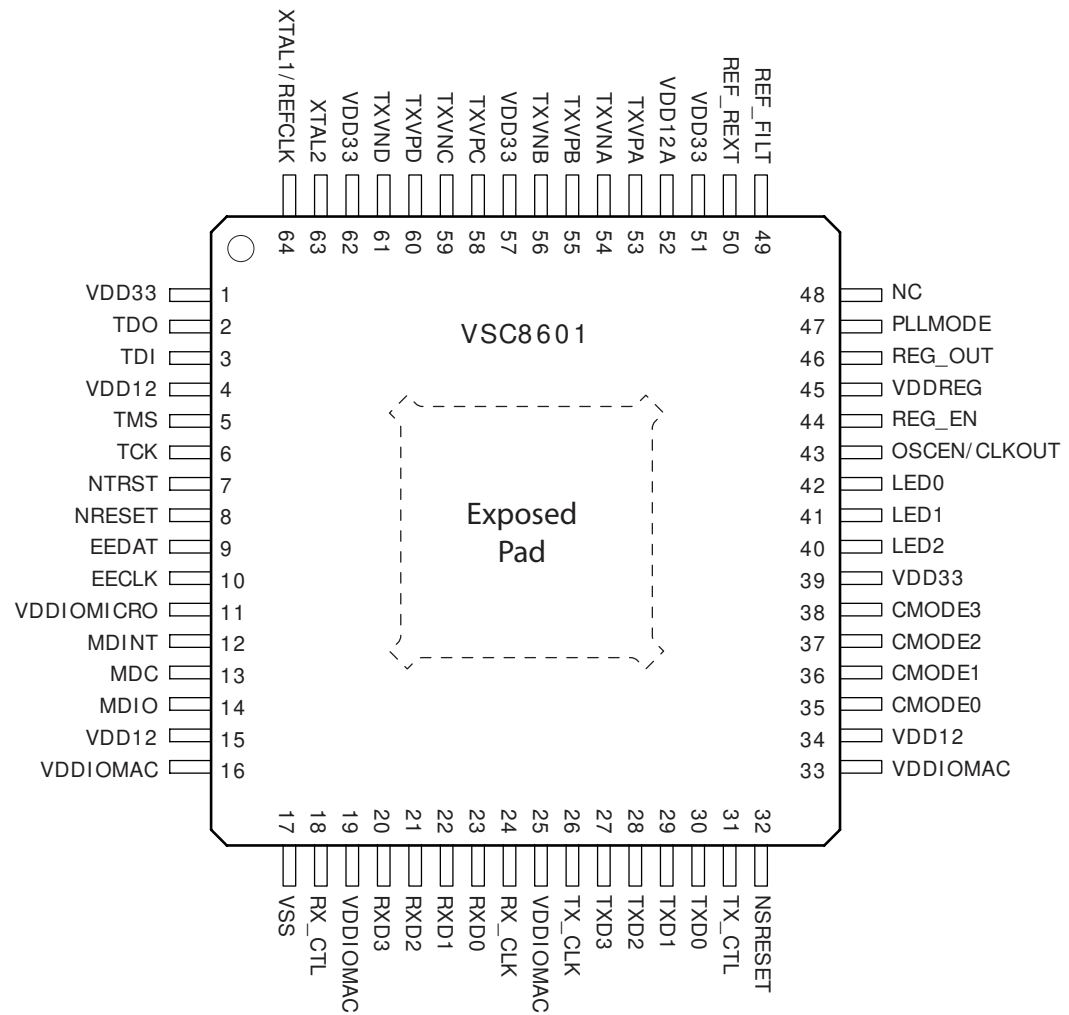
Figure 23. Pin Diagram
