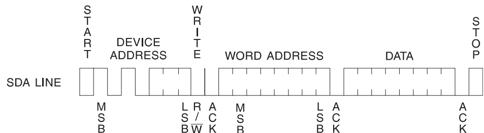
Figure 11. Byte Write
