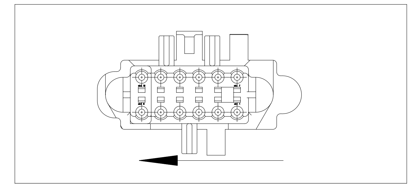
RECEPTACLE SLIDES INTO MOUNTED POSITION
