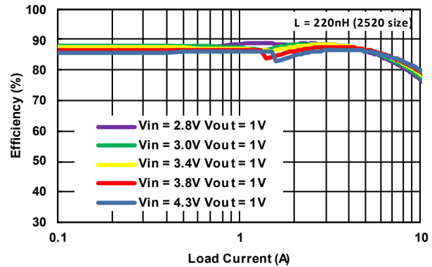
Figure 7. Dual-Phase Efficiency ( V_{OUT} = 1V ), Continuous Load Sweep (0.1A to 10A)
