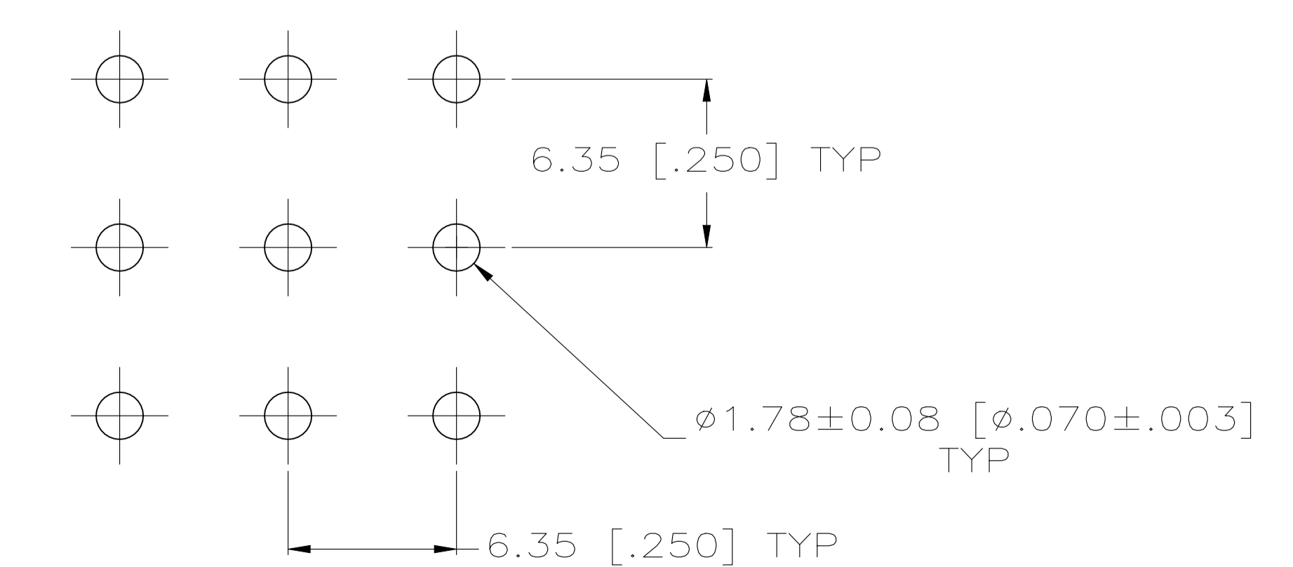
RECOMMENDED LAYOUT FOR 1.58 [0.062] THICK PC BOARD
