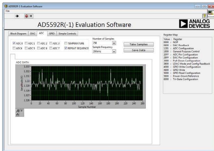
Figure 8. ADC Tab
