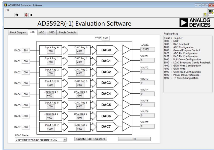
Figure 7. DAC Tab
