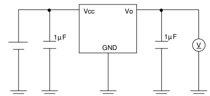
Measurement Circuit of Figure 12 and Figure 21
