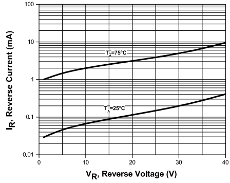
Leakage Current
