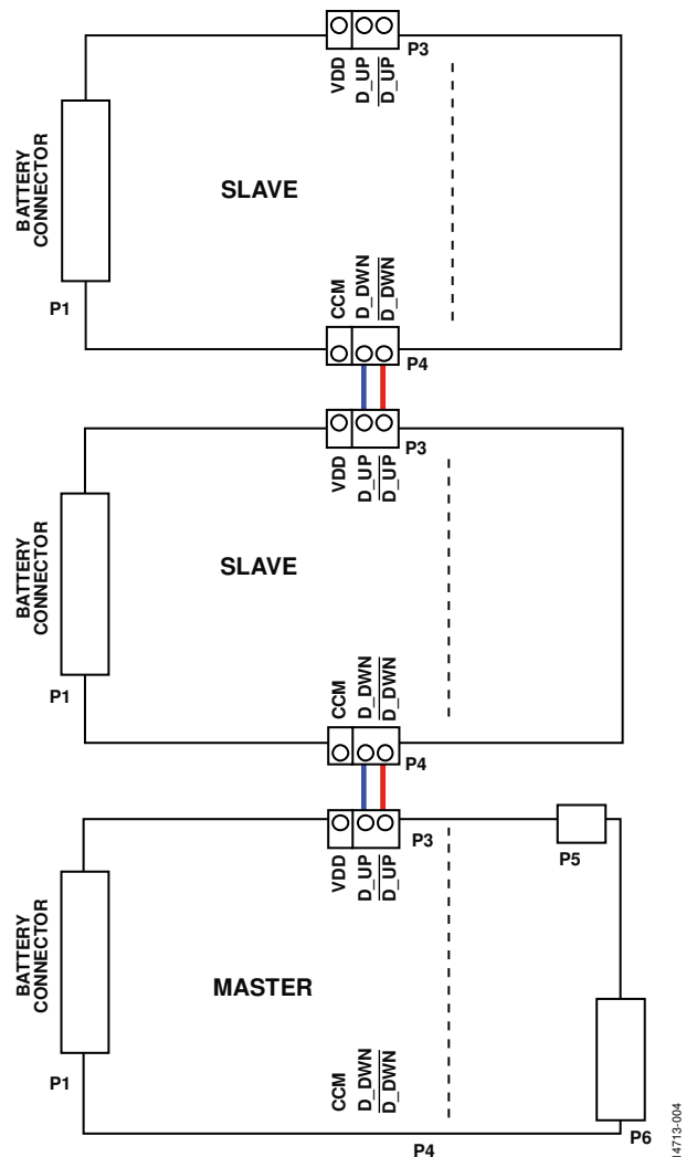
Figure 4. Direct Current Daisy-Chain Configuration of Master with Two Slaves for Direct Current Daisy-Chain Configuration
