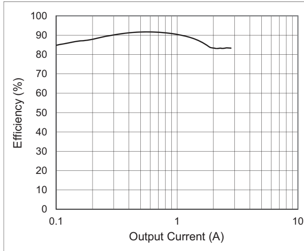
Figure 6. Boost - Efficiency vs. Output Current; V IN = 24V
