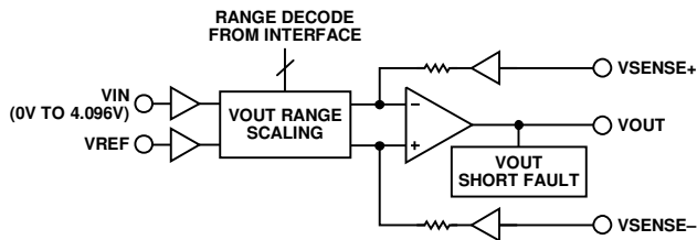
Figure 54. Voltage Output
