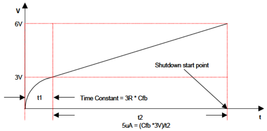
Figure 25. Delayed Shutdown
