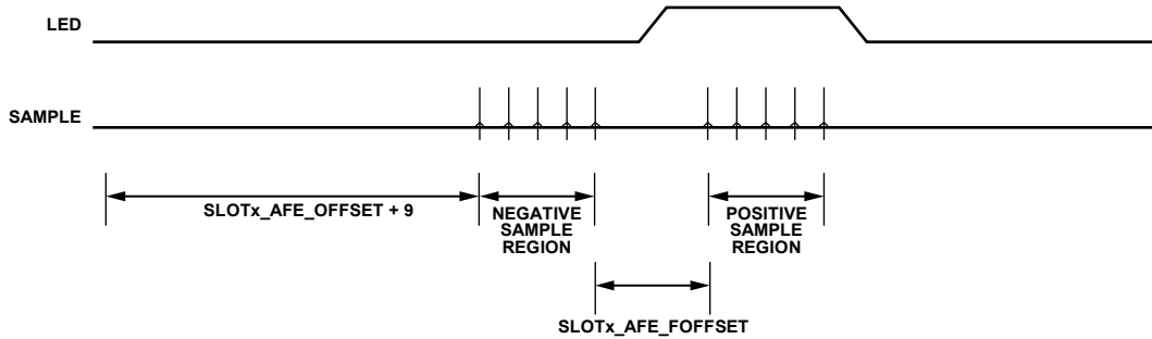
Figure 48. Digital Integration Mode in Single-Sample Pair Mode with Gapped Sample Timing
