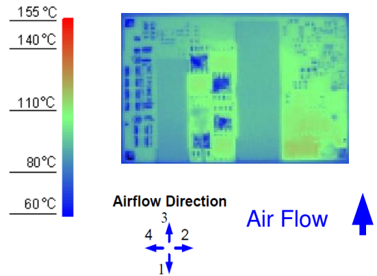
Figure 10. Thermal Image for Airflow Direction 3 (49A output, 75°C ambient, 200 LFM, typical V_{in} , open frame, soldered interface)
