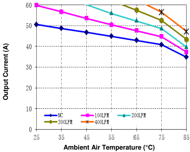
Figure 9. Current Derating Curve for Airflow Direction 3 (Ref. Fig. 10 for Airflow Direction; typical V_{in} , open frame, soldered interface)
