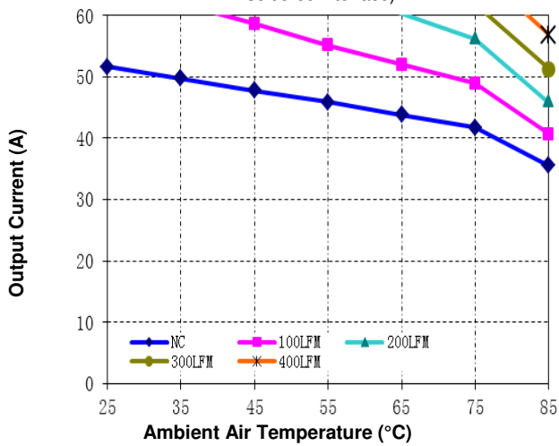
Figure 11. Current Derating Curve With Baseplate
