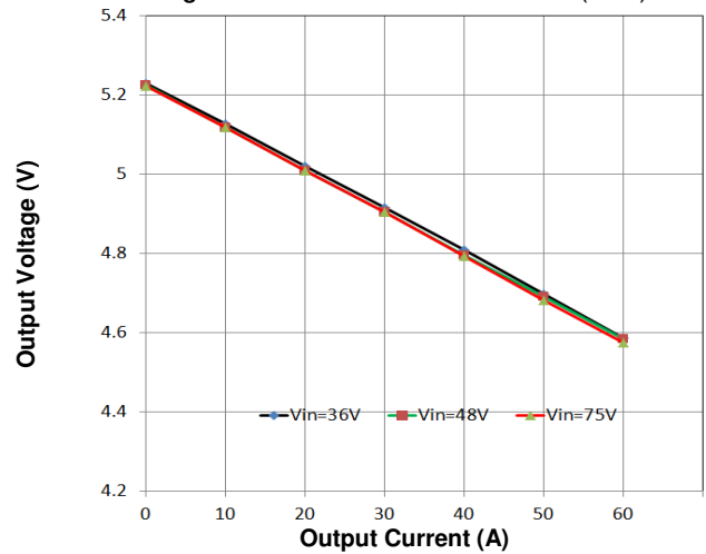
Figure 4. Output Characteristics (parallel option)
