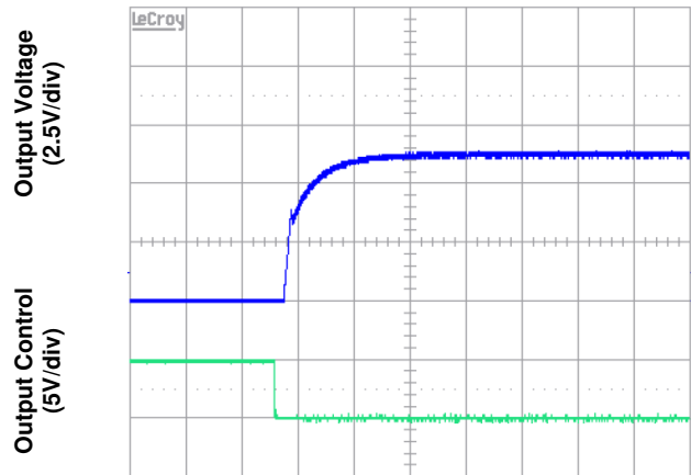
Figure 6. Start-Up from Enable Control (typical Vin, zero load, external Cap.=1000µF)
