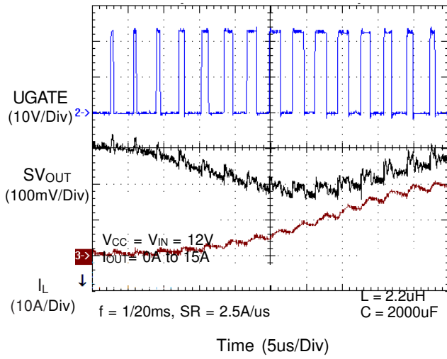
Transient Response (Rising)
