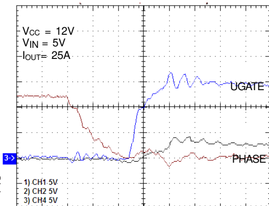
Dead Time (Rising)
