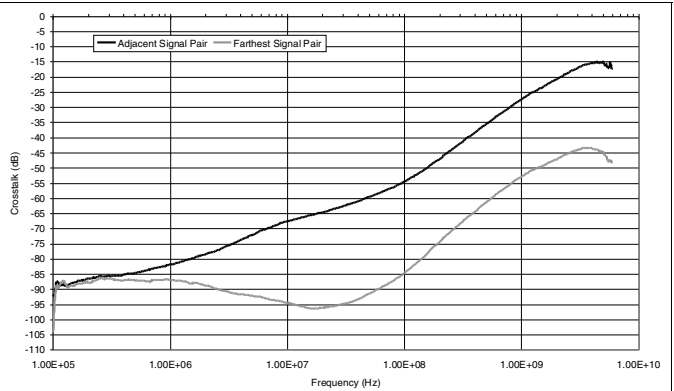
Figure 8. TPD6F003
