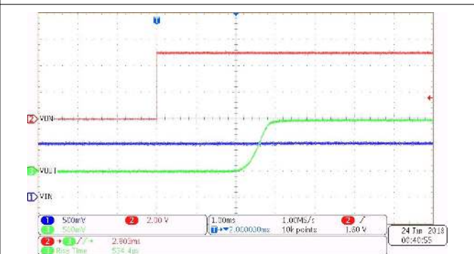
Figure 7-18. Turn-On at 1 V (CT = 1000 pF)
