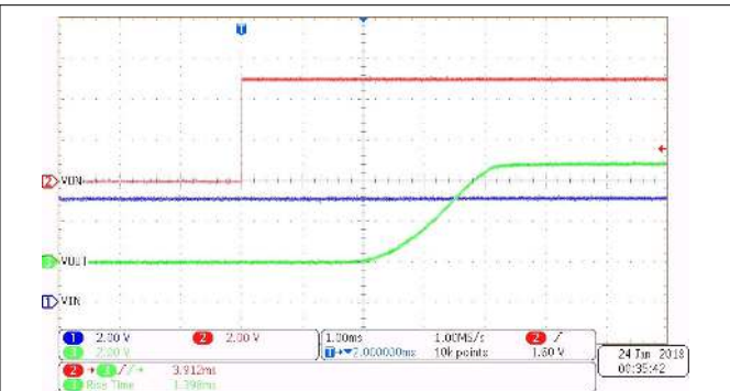
Figure 7-14. Turn-On at 5 V (CT = 1000 pF)
