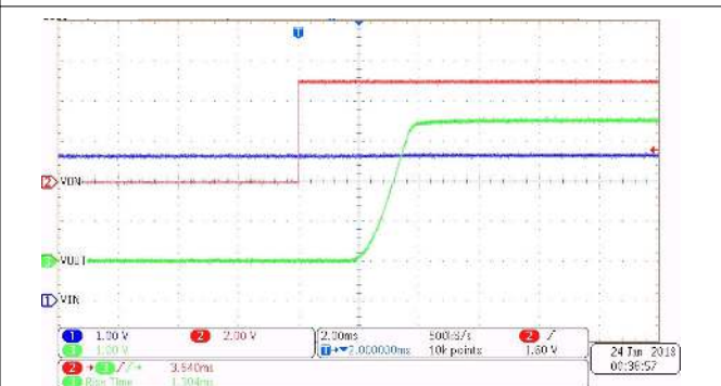
Figure 7-16. Turn-On at 3.6 V (CT = 1000 pF)
