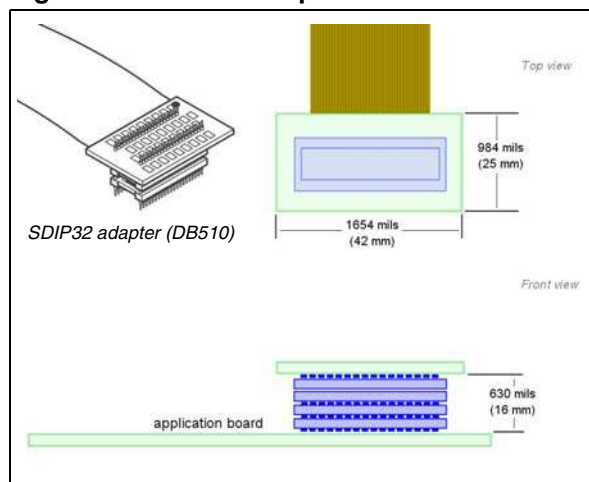
Figure 1. SDIP32 adapter
