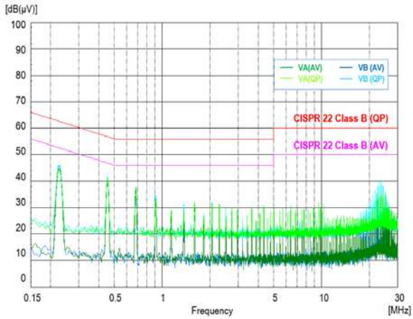
Conduction Noise (Vin=48V, Iout=2.125A, Ta=+25°C) with External Input Filter
