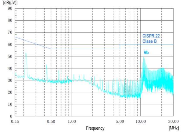
Conduction Noise ( V_{in}=48V , I_{out}=5.1A , T_a=+25^{\circ}C ) with External Input Filter
