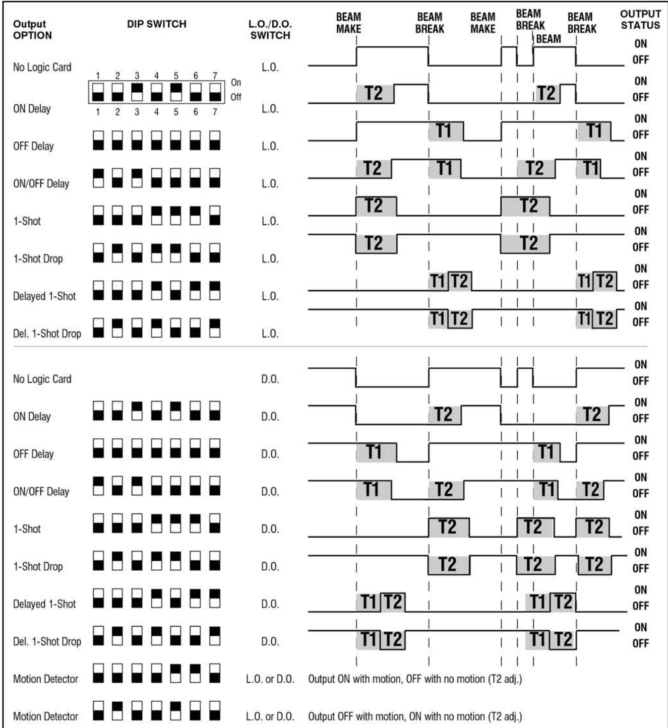
DIP SWITCHES 1-7
