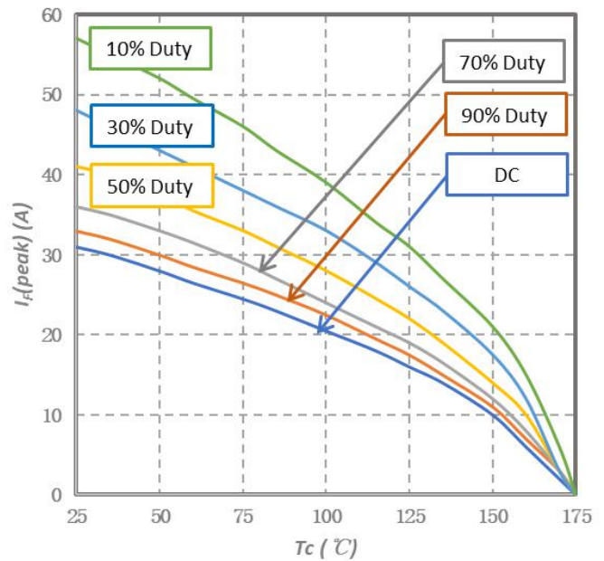
Fig.8-Current Derating
