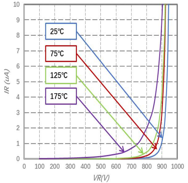
Fig.2-Typical Reverse Characteristics
