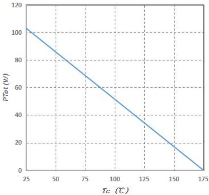
Fig.7-Power Derating
