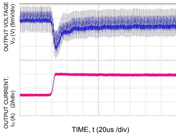
Figure 48. Transient Response to Dynamic Load Change from 50% to 100% at 12Vin, Cout=1x47uF + 4x330uF, CTune=33nF, RTune=178
