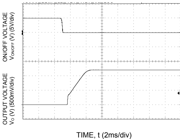
Figure 43. Typical Start-up Using On/Off Voltage (Io = Io,max).
