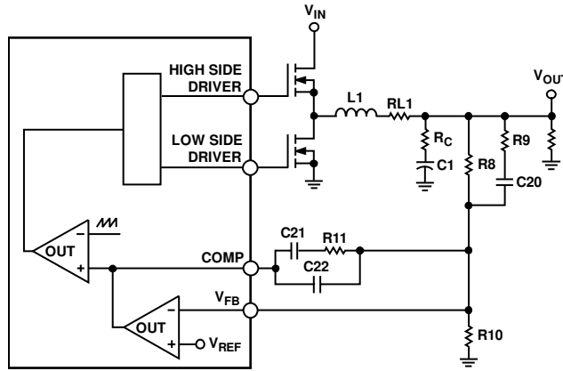
Figure 2. Control Loop
