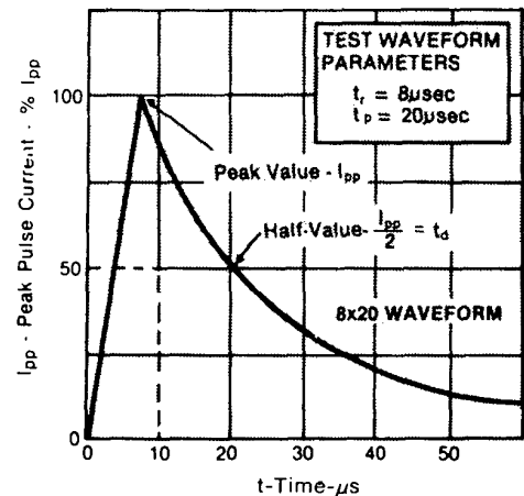
FIGURE 2 Pulse Waveform
