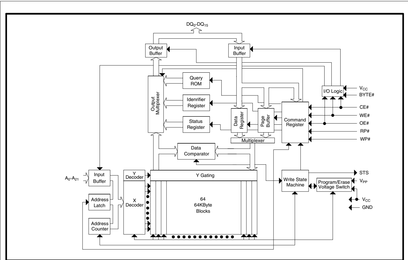
Figure 1. Block Diagram
