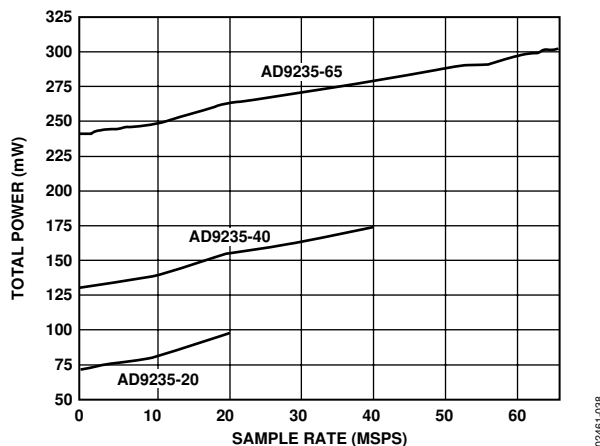
Figure 38. Total Power vs. Sample Rate with f_N = 10 MHz
