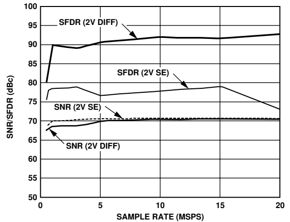
Figure 14. AD9235-20: Single Tone SNR/SFDR vs. f_{\text{CLK}} with f_{\text{IN}} = \text{Nyquist} (10 MHz)
