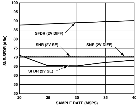
Figure 13. AD9235-40: Single Tone SNR/SFDR vs. f_{\text{CLK}} with f_{\text{IN}} = \text{Nyquist} (20 MHz)
