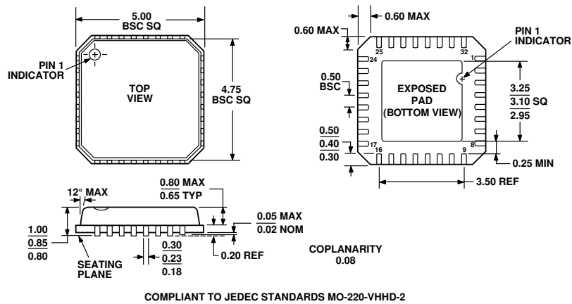
Figure 64. 32-Lead Lead Frame Chip Scale Package [LFCS] 5 mm × 5 mm Body (CP-32-2) Dimensions shown in millimeters
