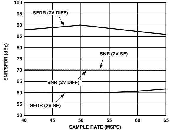
Figure 12. AD9235-65: Single Tone SNR/SFDR vs. f_{\text{CLK}} with f_{\text{IN}} = \text{Nyquist} (32.5 MHz)
