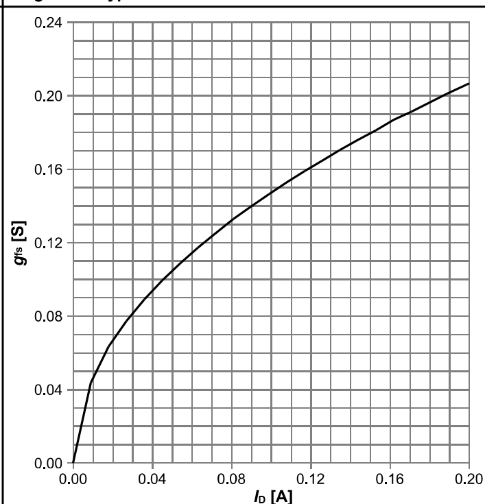
Diagram 8: Typ. transconductance
