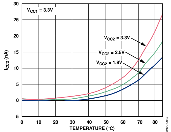
Figure 10. I_{CC2} vs. Temperature
