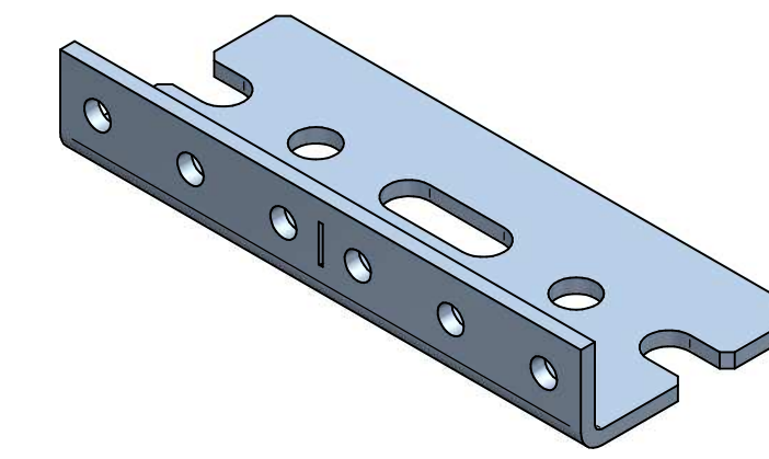
ISOMETRIC
